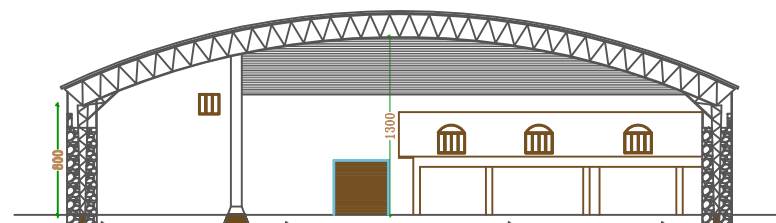
EXHIBITION HALL SECTION EXHIBITION HALL - 1
